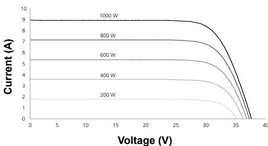
I-V Curve S 250M60 Vision black
