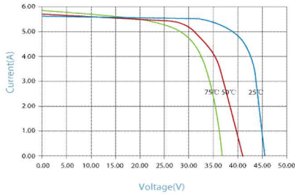
IV-CURVES of PV module SL195TU-36MBK
