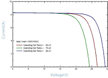
IV-CURVES of PV module SL180TU-24P
