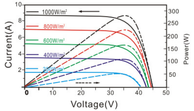
I-V Curves at different Irradiances Test temperature: 25°C
