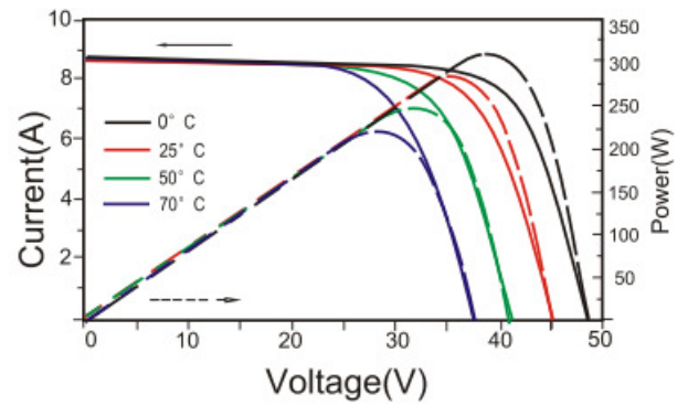
Irradiance: AM1.5, 1000W/m²
