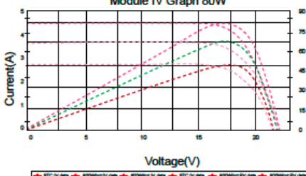
Module IV Graph 80W
