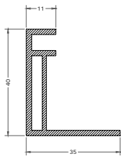
Frame cross section
