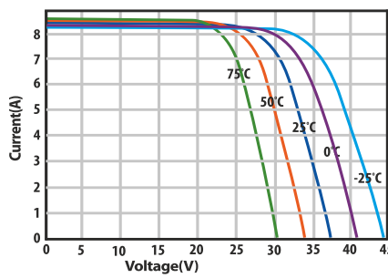
TEMPERATURE IV CURVES OF USP-P6-60
