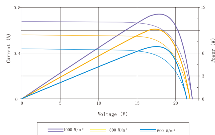
10W PV I-V characteristic curves
