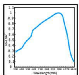
Spectral Response
