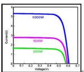
IV-Curve
