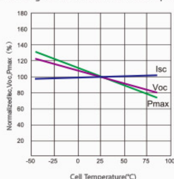
Power voltage current curve at different temperature
