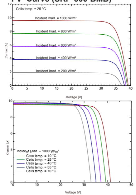
I-V Curve (SRP-300-BMB)
