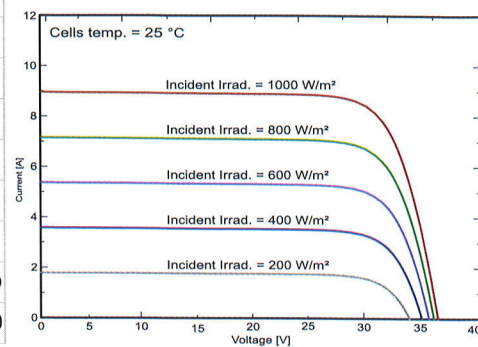
IV Curves for 305 Wp monocrystalline module
