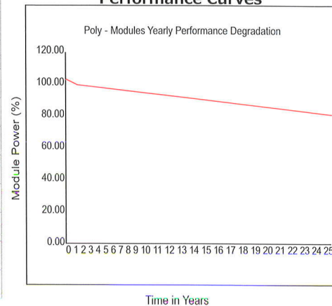
Performance Curves
