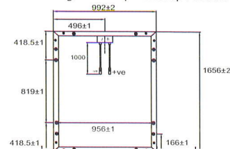
Drawing of 290Wp - 310Wp Module
