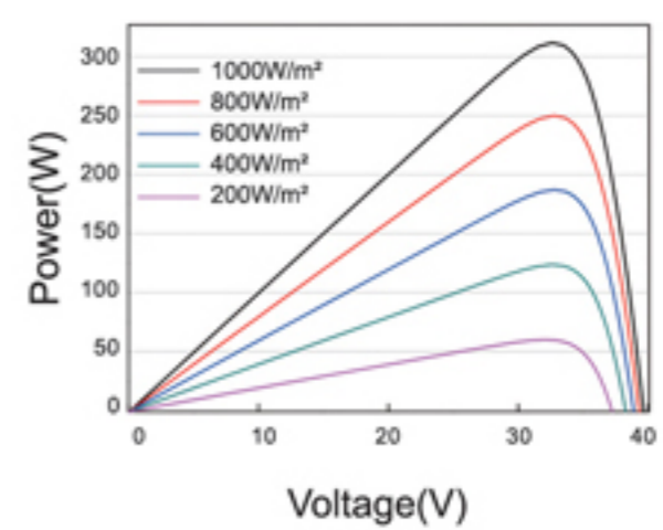
Power-Voltage Curve DHM60H-305
