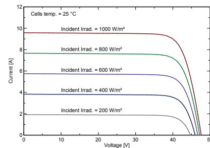
I-V Curve (SRP-355-BMA(-HV))
