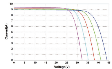
Current-Voltage Curves at Different Temperatures
