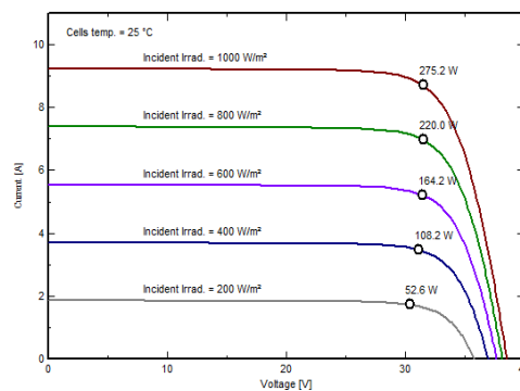
I-V Curve of 275W at 25°C cell temp. and different Irradiance level
