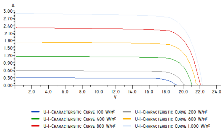
U-I-CHARACTERISTIC CURVE AT 25 °C
