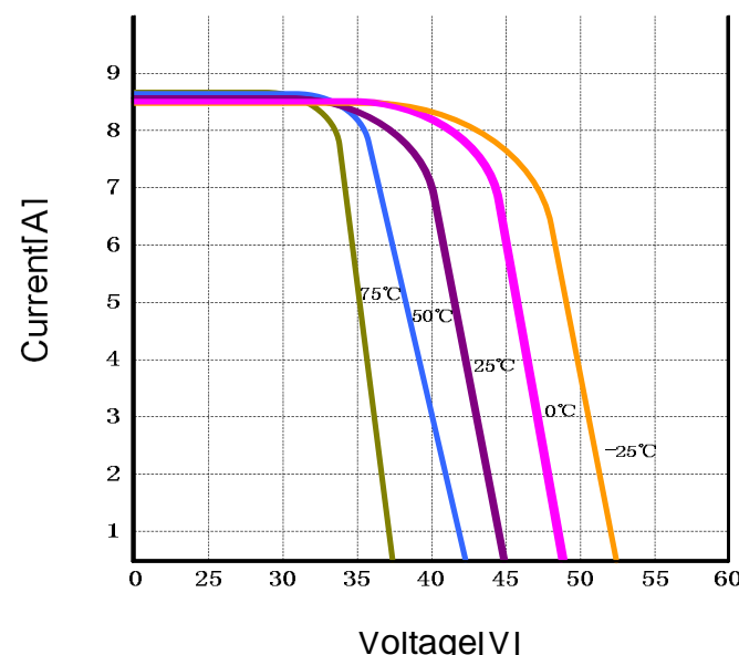
Module characteristics at different module temperatures and constant Module irradiance(1.000W/m²).
