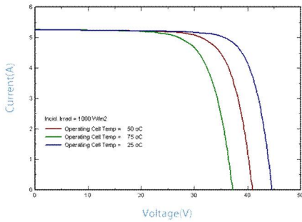
IV-CURVES of PV module RD165TU-36SP
