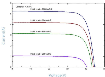
IV-CURVES of PV module RD190TU-36SP
