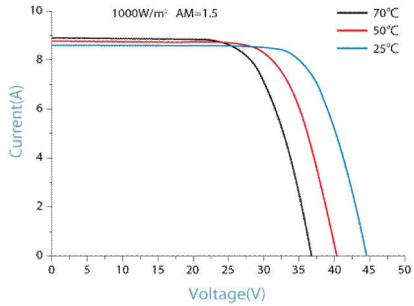
IV-CURVES of PV module RD290TU-36P
