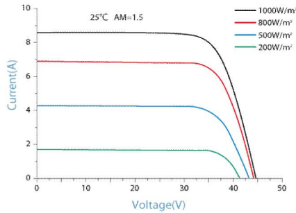
IV-CURVES of PV module RD290TU-36P
