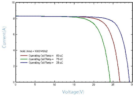
IV-CURVES of PV module RD200TU-24MD
