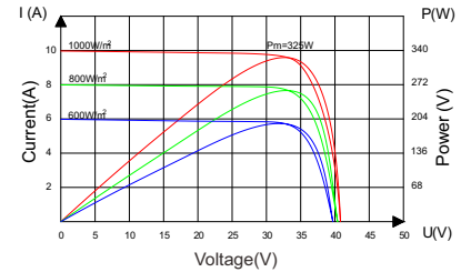
Current-Voltage&Power-Voltage Curve(325W)
