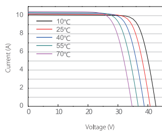
Current-Voltage Curve(AOX-60MS-345W)
