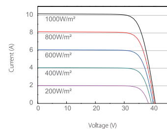
Current-Voltage Curve(AOX-60MS-345W)
