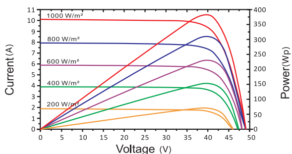
I-V characteristics at different irradiances. Current-Voltage & power Voltage Curve (390)
