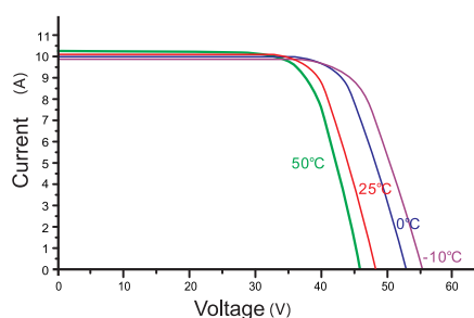
I-V characteristics at different temperature (AM1.5, 1000W/m²)
