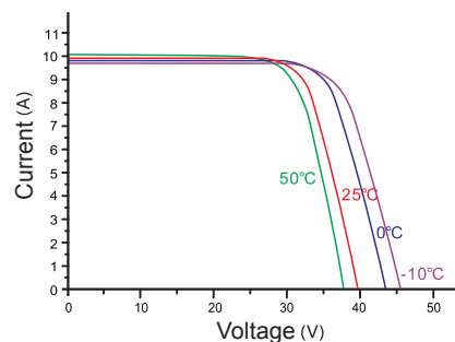
I-V characteristics at different temperature (AM1.5, 1000W/m²)
