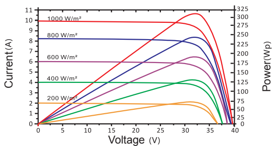
I-V characteristics at different irradiations. Current-Voltage & power Voltage Curve (325)
