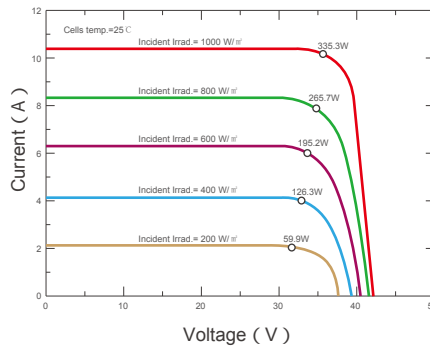
Current-Voltage & Power-Voltage Curves (RMHB60-335S1)
