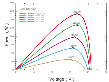
Current-Voltage & Power-Voltage Curves (RMHB60-335S1)
