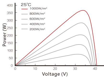
Power curve under different irradiance OLV-365-60M-DC9H
