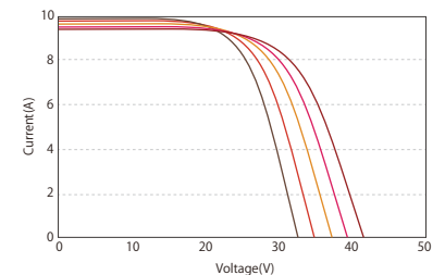
U-I Curve at Different Temperature (305W)
