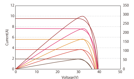
U-I/P-U Curve at Different Irradiation (305W)
