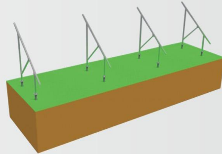
2 Leg Pipe, square Pipe and Beam Rail Installation
