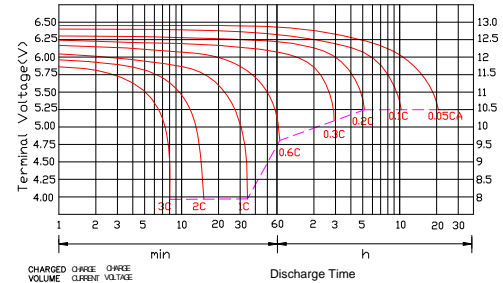
DISCHARGE CHARACTERISTICS AT 25; 6(77; 5)
