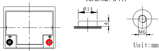
Terminal (F11)
