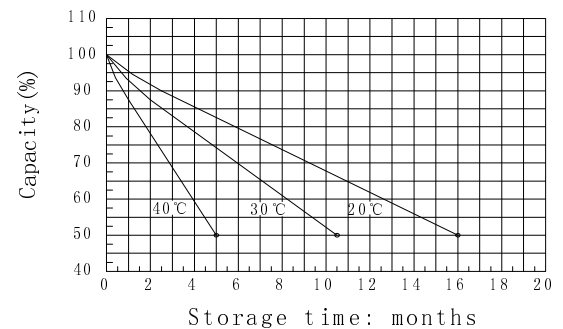
Self-discharge characteristic
