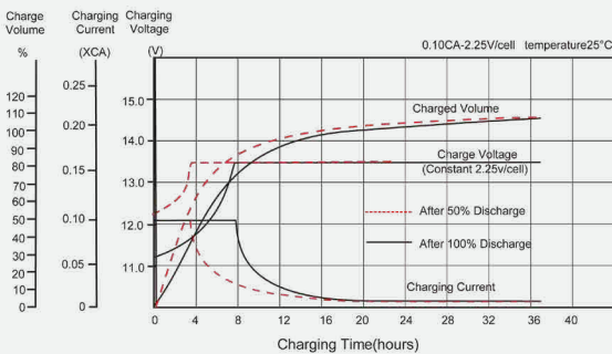
充电曲线 Charge Characteristics
