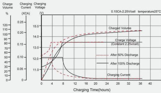
充电曲线 Charge Characteristics
