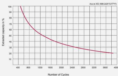
循环次数曲线 Cycle Life Characteristics
