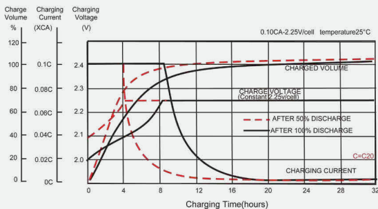
充电曲线 Charge Characteristics
