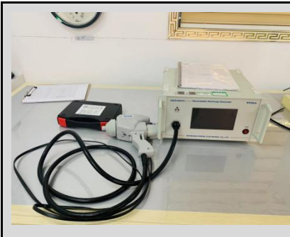
Electrostatic Discharge Generator (ESD-DESK)
