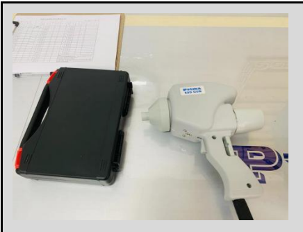
Electrostatic Discharge Generator (ESD61002TC)
