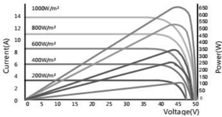
IV-Curves
