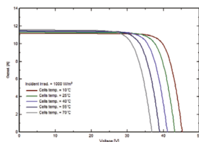
I-V Curve at different temperature (SPP385QHEH)
