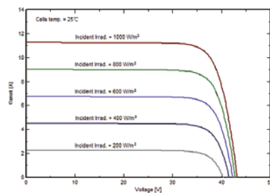
I-V Curve at different irradiation (SPP385QHEH)
