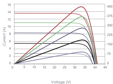
Current-Voltage Curve (TP120-450M/MB-8)
