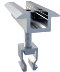
Mid-Clamp Set
