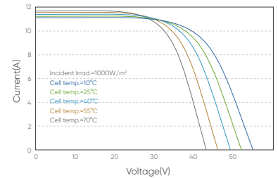
I-V Curve at Different Temperature (465W)
