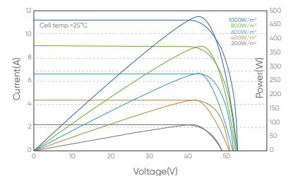
I-V/P-V Curve at Different Irradiation (465W)
