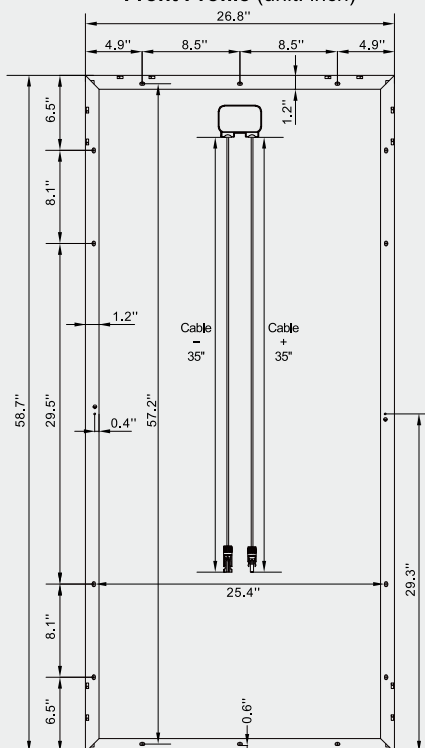
Back Profile (unit: inch)
