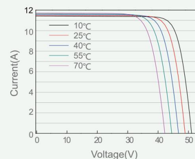
Current-Voltage Curve(SP455M-72H)
