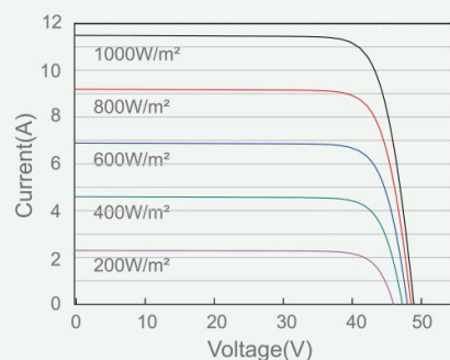
Current-Voltage Curve(SP455M-72H)
