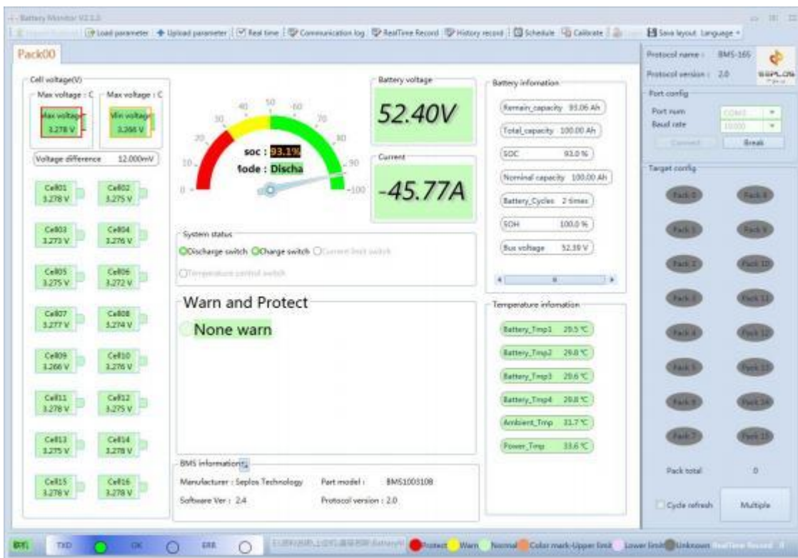
Software interface
