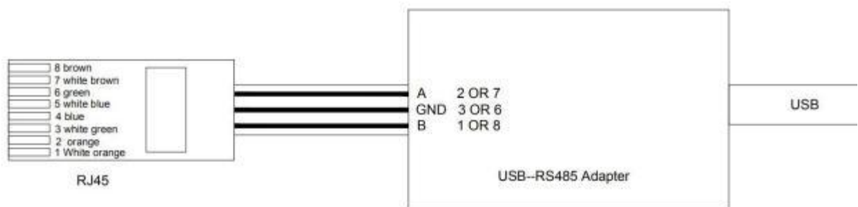
Wiring Diagram
