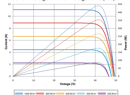
Current-Voltage & Power-Voltage Curve (450)
