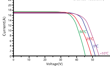
I-V characteristics at different temperatures
