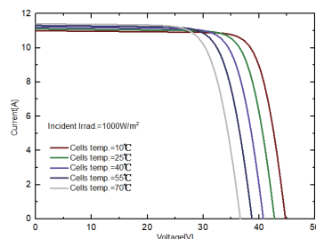
I-V Curves of FLEX370B at different cell temperature
