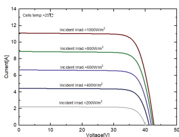
I-V Curves of FLEX370B at different irradiance
