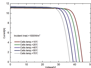
I-V Curves of FLEX375A at different cell temperature
