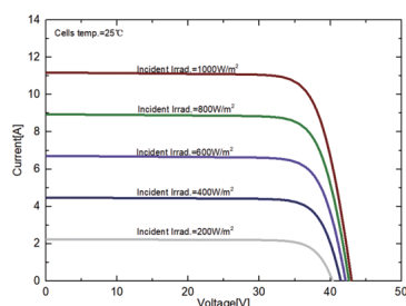
I-V Curves of FLEX375A at different irradiance
