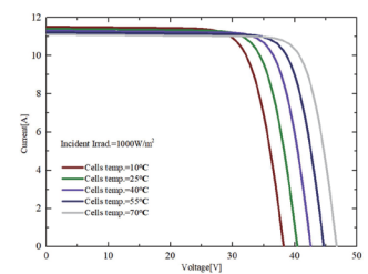
I-V Curves of PERC395 at different cell temperature
