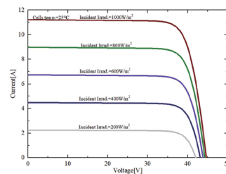
I-V Curves of PERC395 at different irradiance
