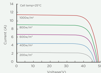
Current-Voltage Curve(SP445M-72H)
