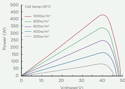
Current-Voltage Curve(SP445M-72H)
