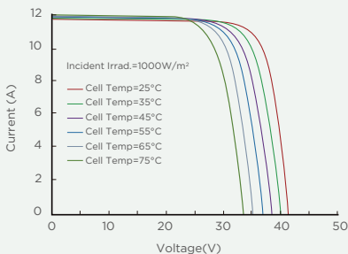
Current-Voltage Curve(SP365M-60H)
