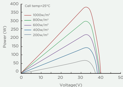
Current-Voltage Curve(SP365M-60H)
