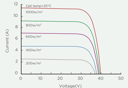
Current-Voltage Curve(SP365M-60H)
